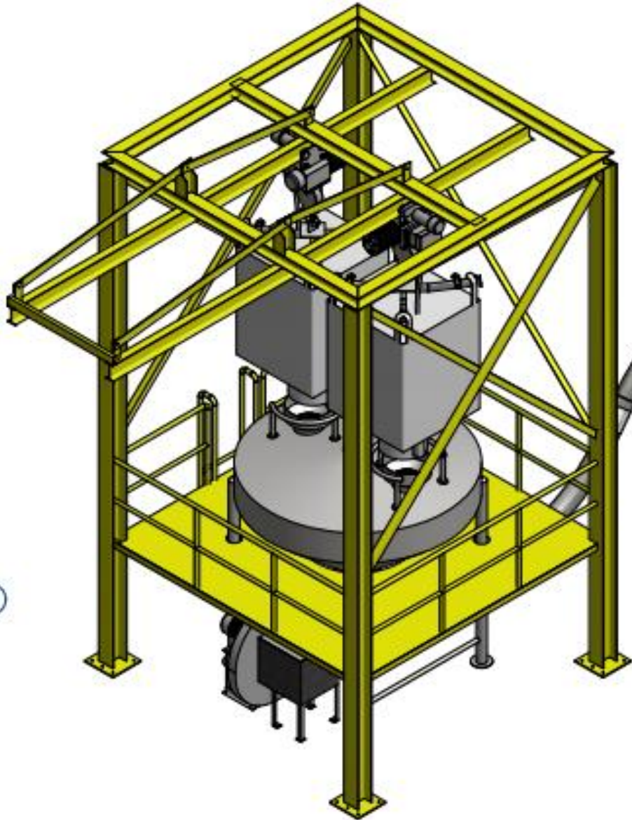
Large Big Bag Unloading Station for Sea Bulk Loader
