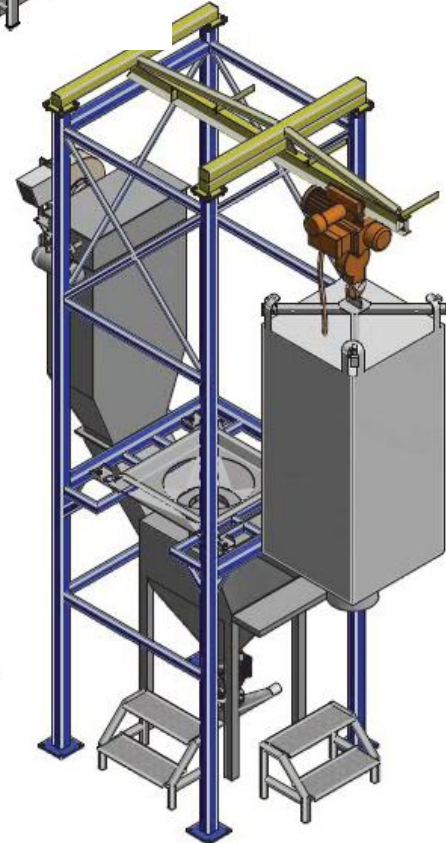
Bag & Bin Unloading Station
